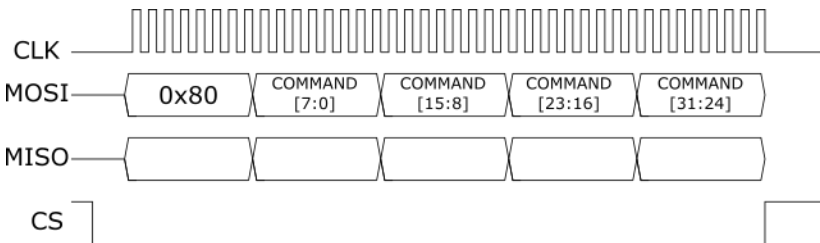
Figure 4: Command Frame
